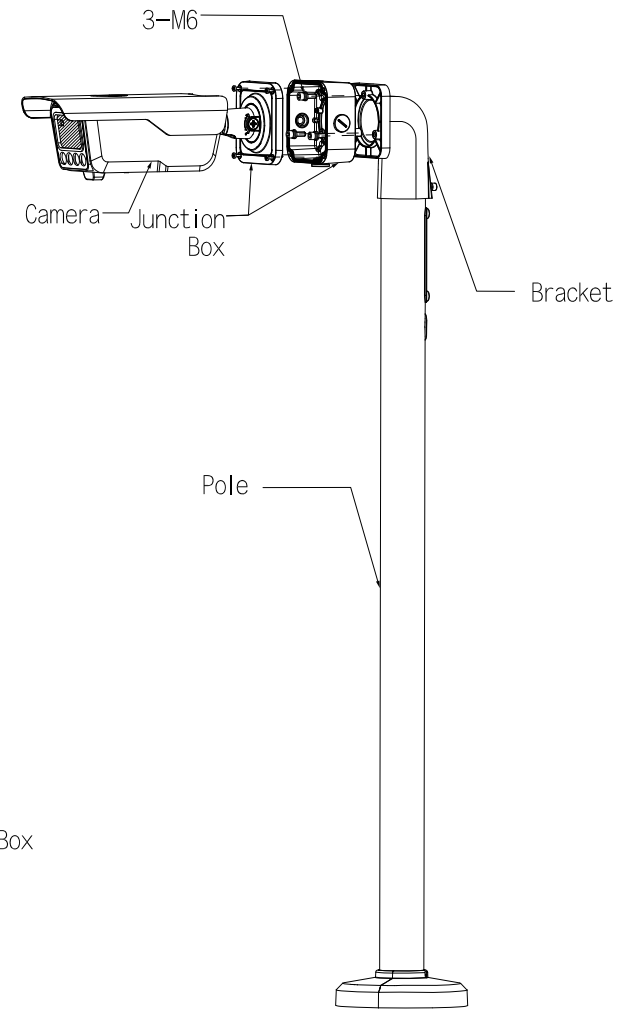
Pole Mount
