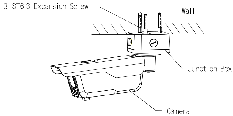
Ceiling Mount
