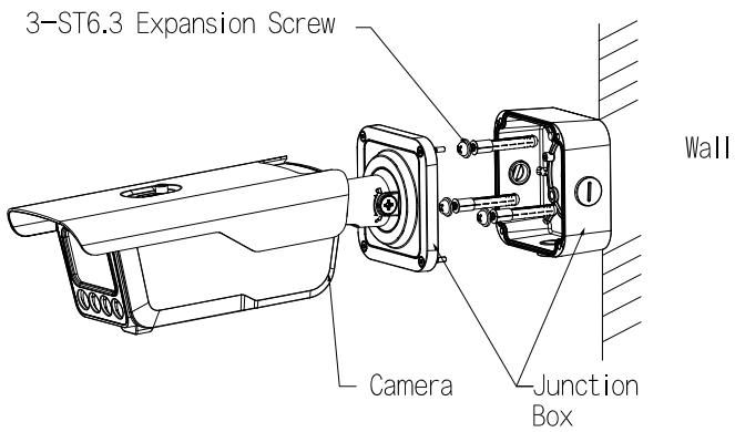
Wall Mount
