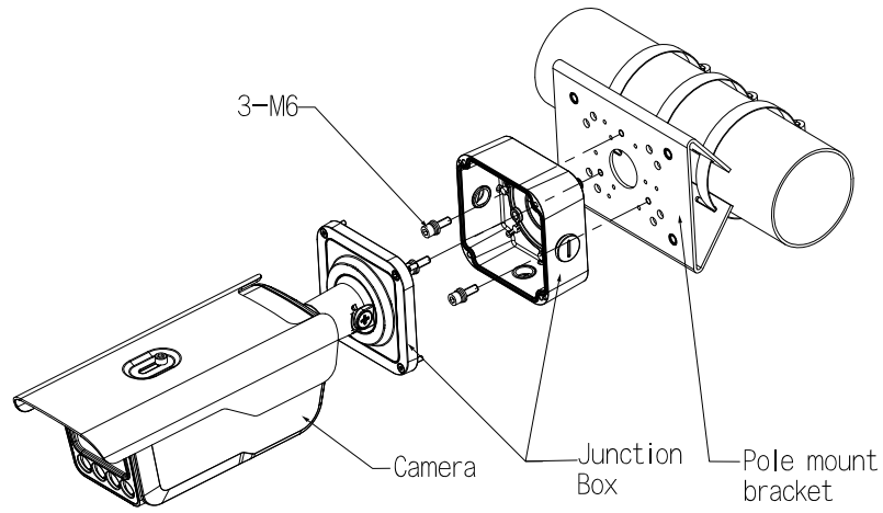
Pole Mount
